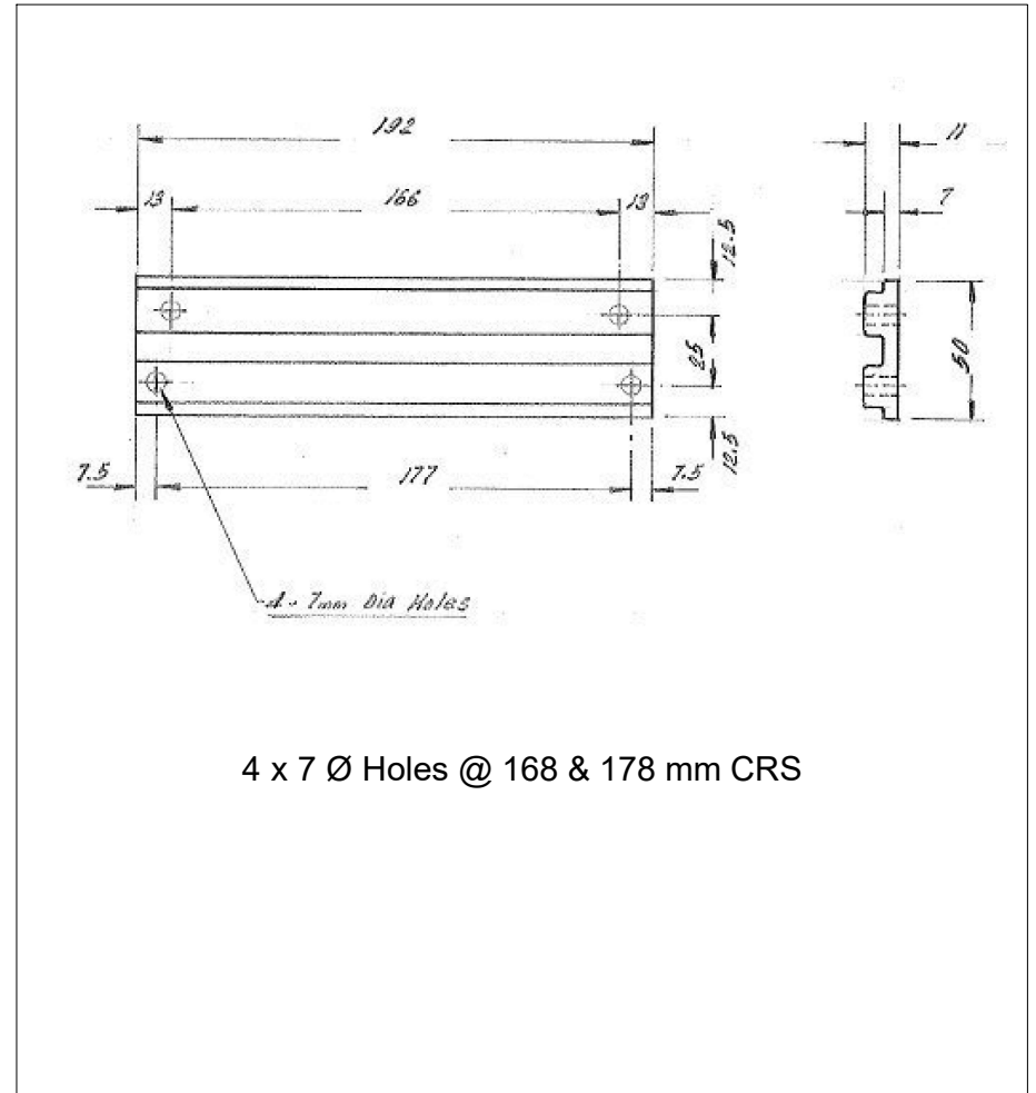
Outboard Plate Anode
