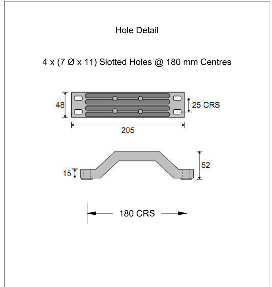
Bracket Anode To Suit 150,200,250 & 300 HP Outboards
