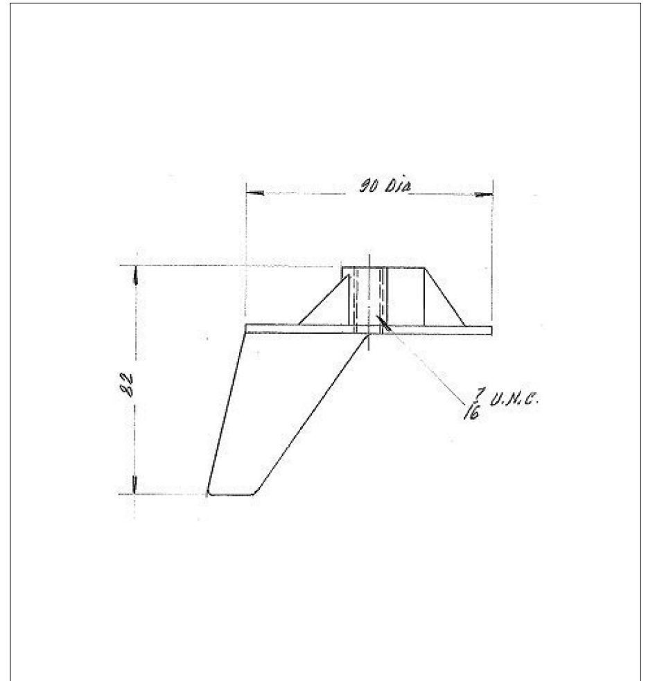
Racing Tab Anode
