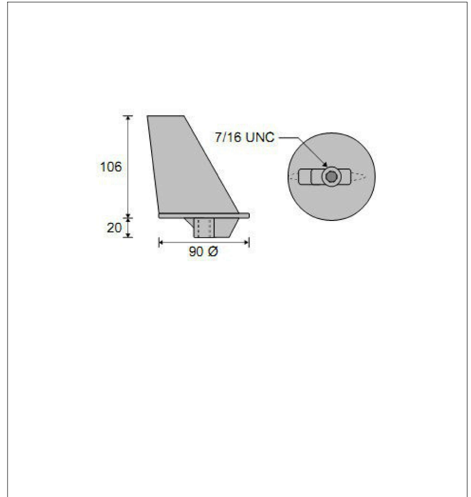
Trim Tab Aluminium Anode - Long Leg
