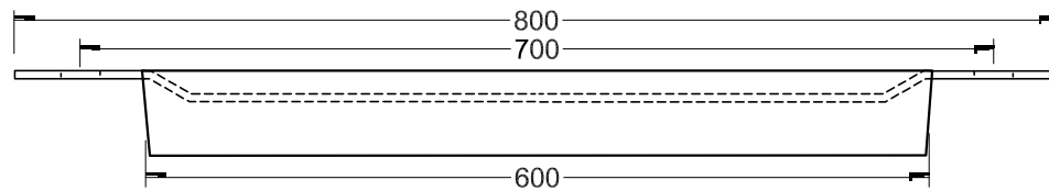
Side View
