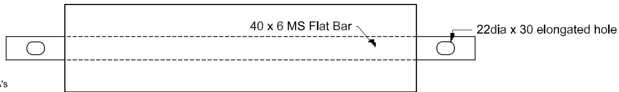
Plan View
