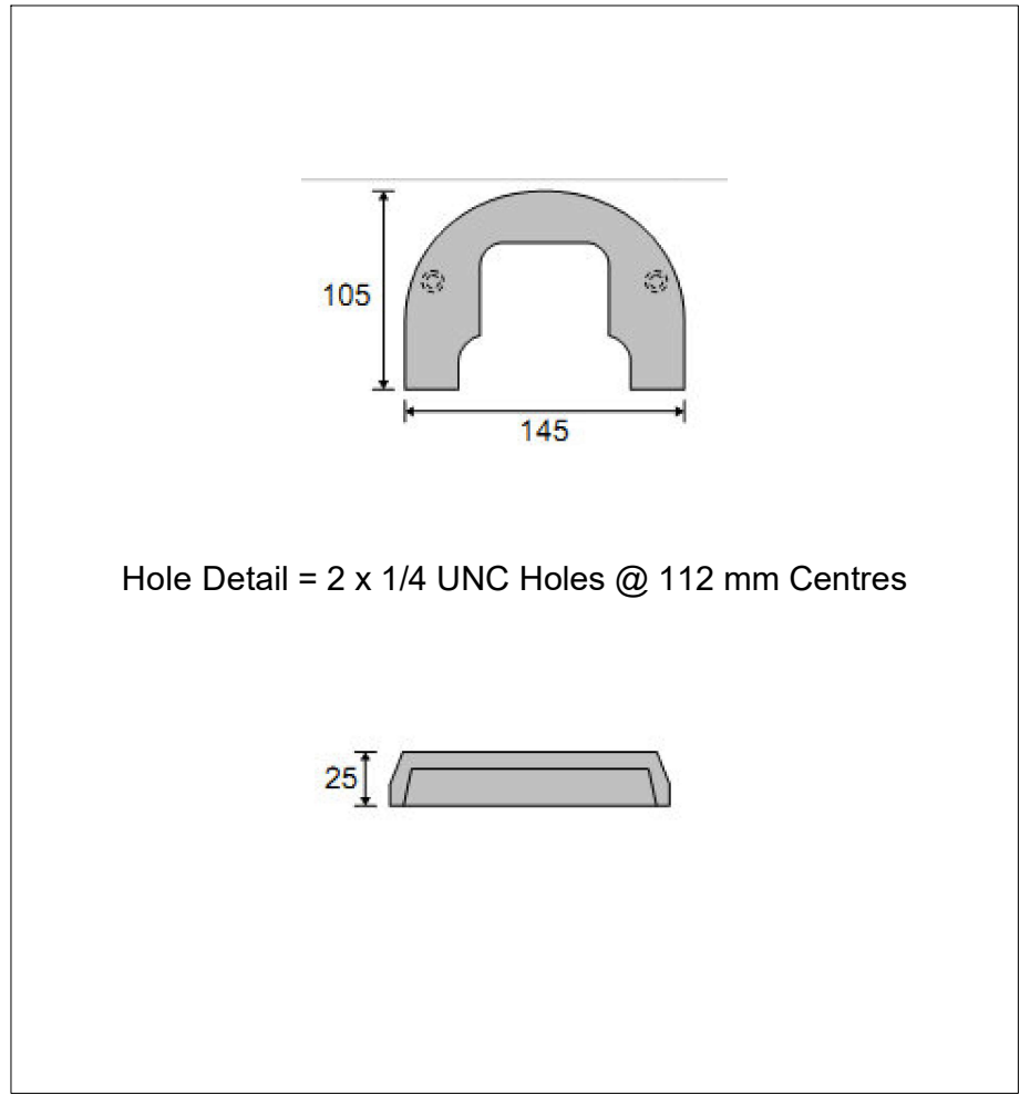
Cobra Horseshoe Anode Replaces Genuine Part: 983494
