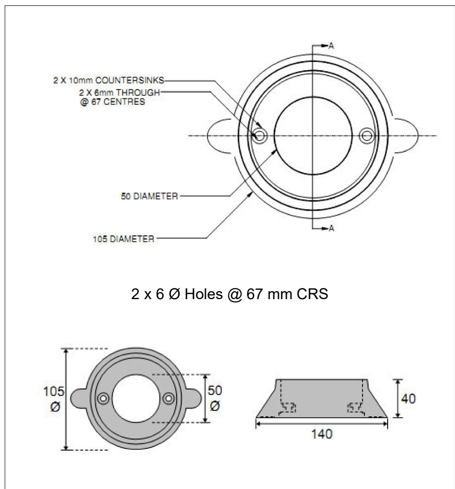
Sail Drive Anode To Suit DV10 Replaces Genuine Part: 024BUK00E5829
