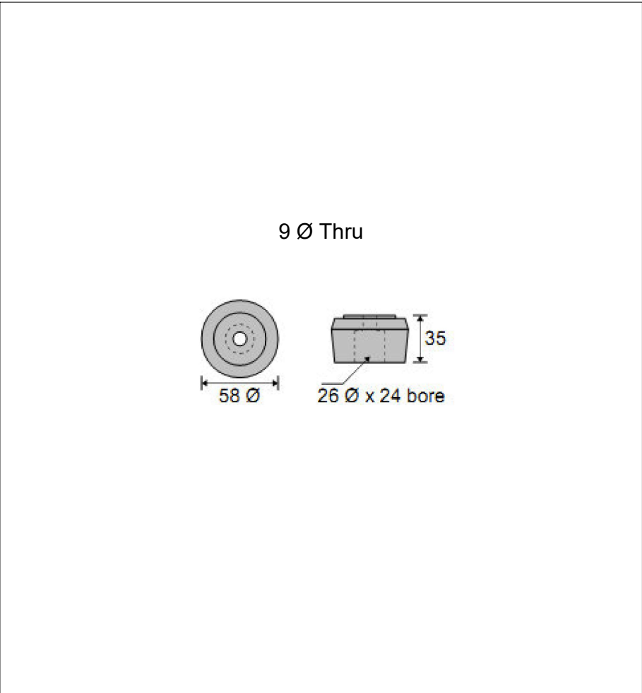
Jet Ring Anode - Small Replaces Genuine Part: 590-16324-3
