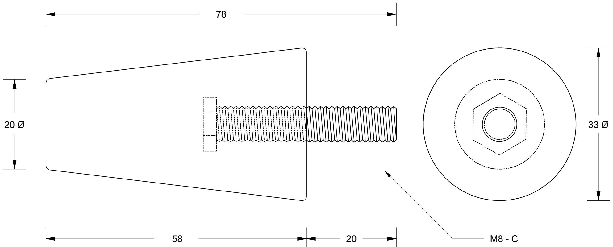
Insert - M8-C (Zinc Plate Hex Set Screw)
