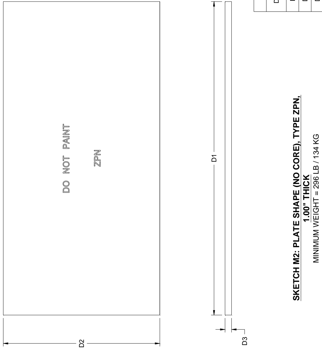
FIGURE 30. Zinc plate shape (no core), type ZPN (1.00" thick)
