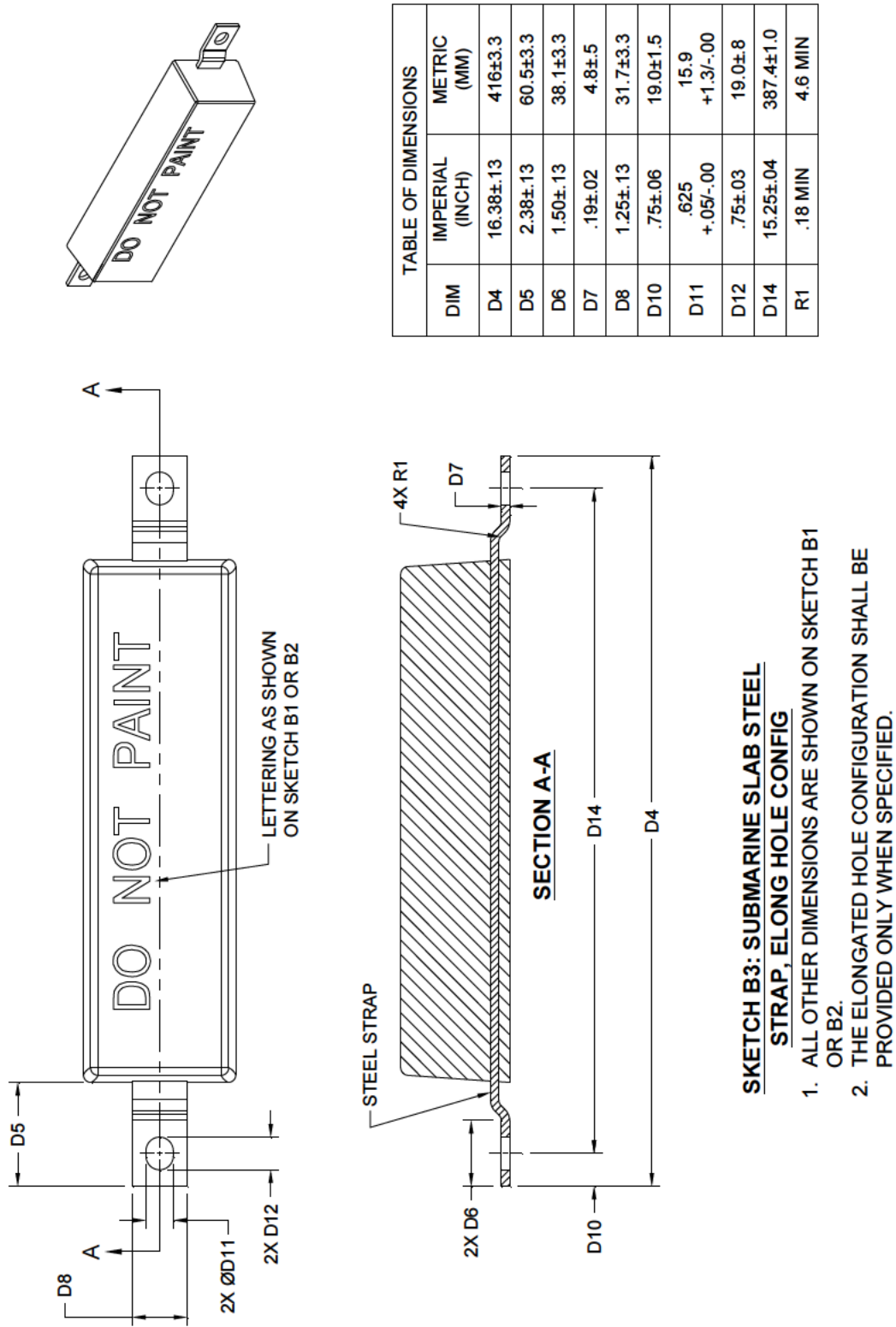
FIGURE 6. Zinc submarine slab (steel strap), type ZSS with elongated stud hole.
